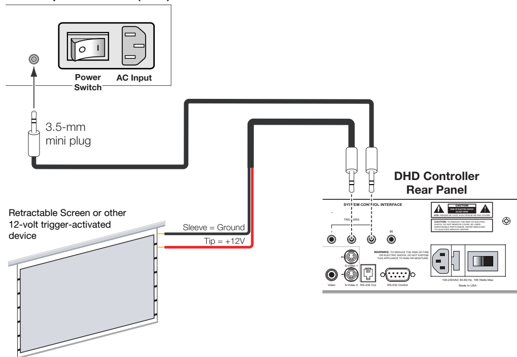
Figure 3-14. Connecting 12-Volt Trigger Outputs
